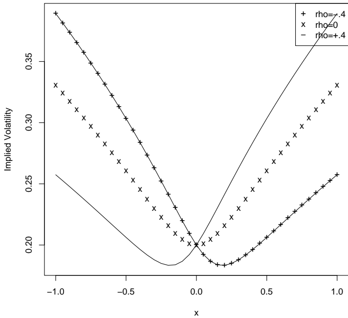
Implied volatility in the small- \epsilon limit
